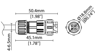
Female connector 4 PIN (IP67)
